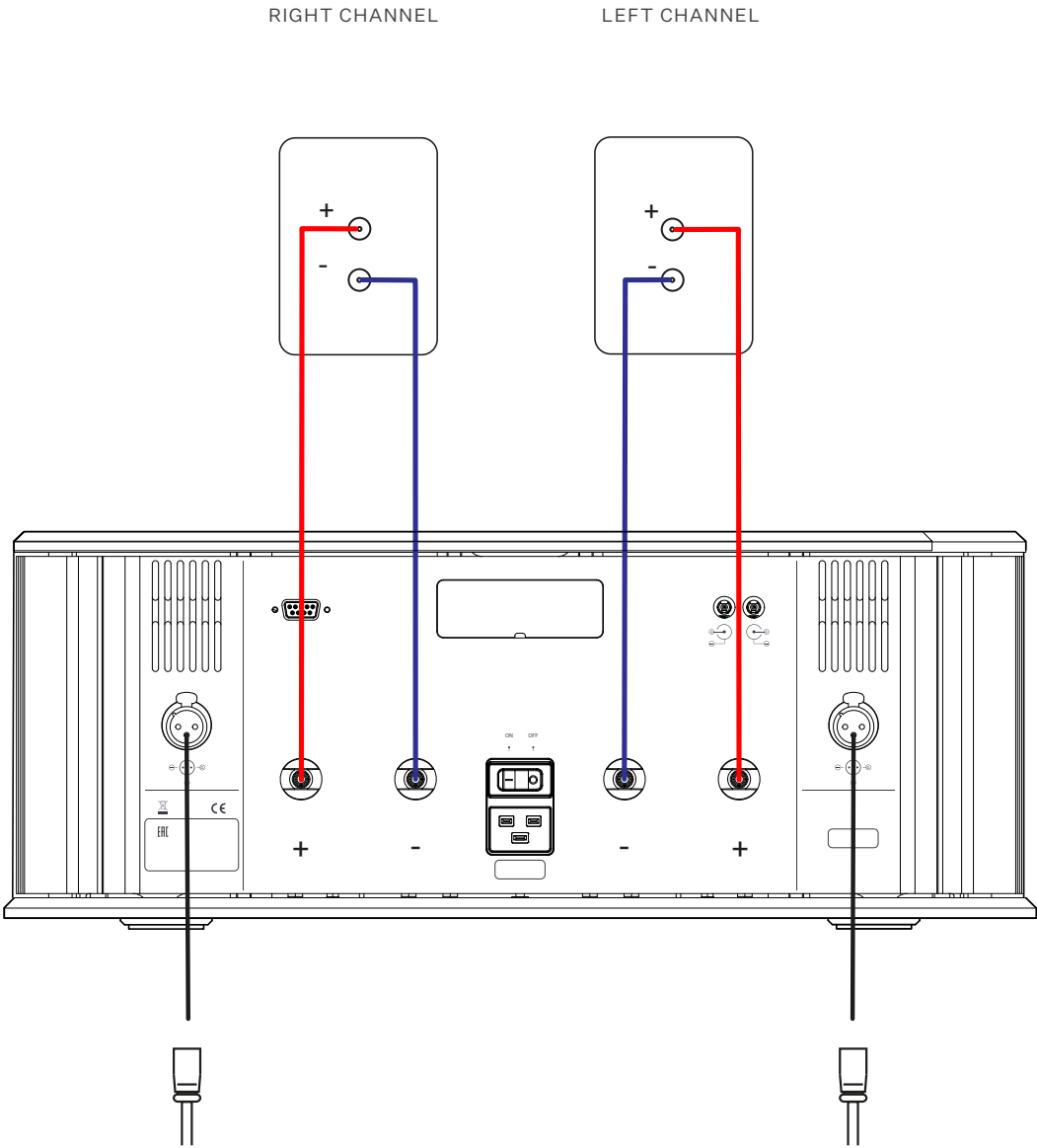
FIGURE 1 STEREO MODE WIRING DIAGRAM
